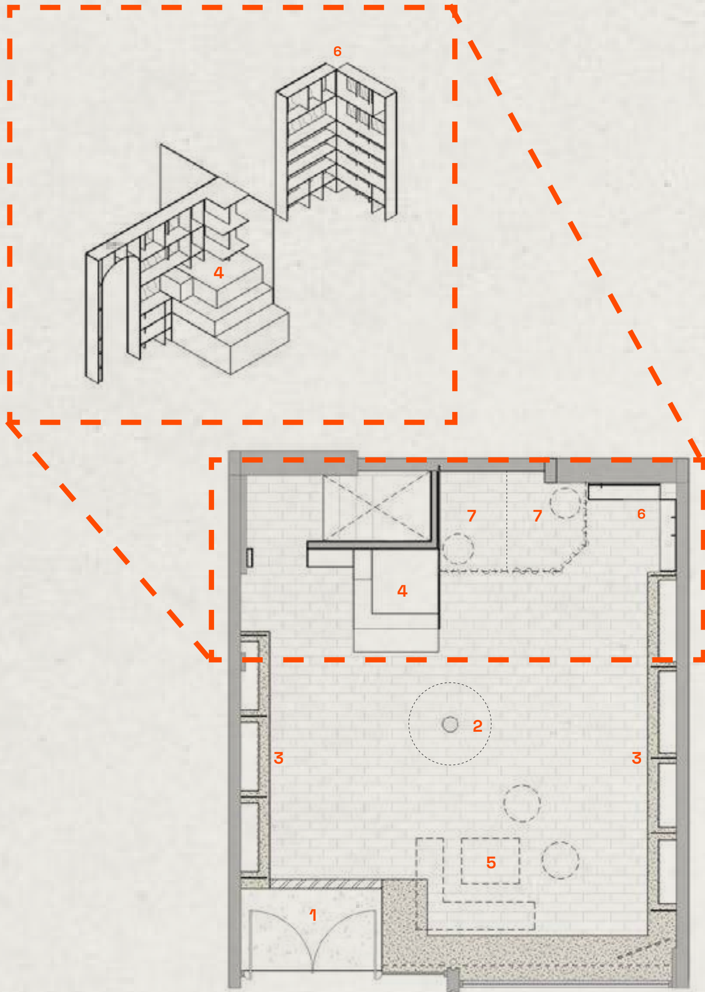
Level 01 | Furniture Plan Note: Plans NTS
